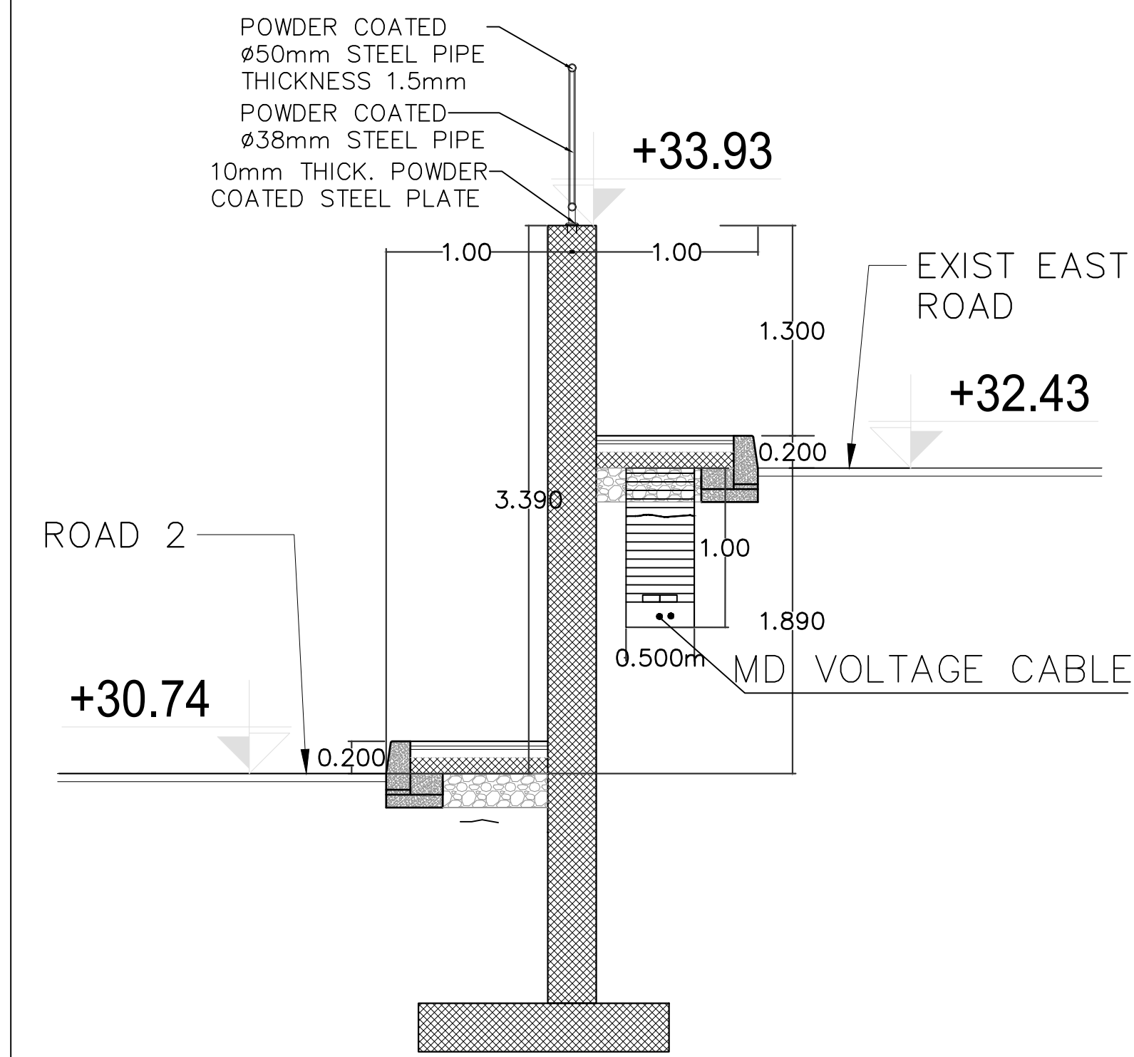
SECTION C
